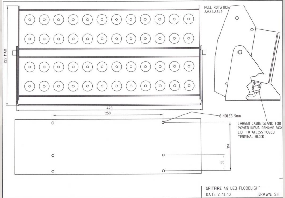
Above: CAD diagram - Spitfire 48 XL110
