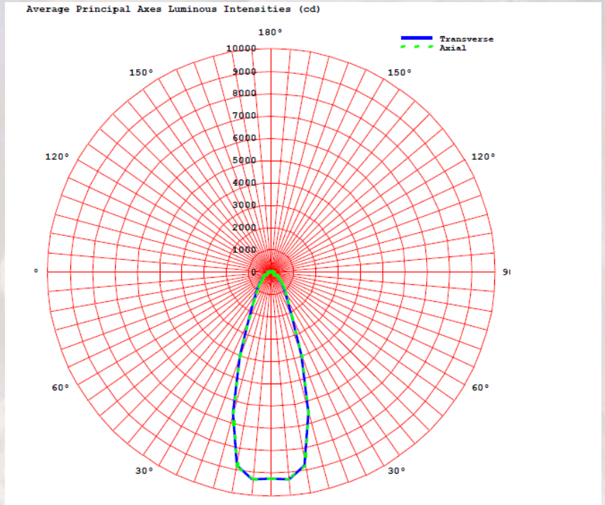
Above: Average Principal Axes Luminous Intensities (cd) - Sovereign 72XL110 – 5 DEGREE MODULE TILT
