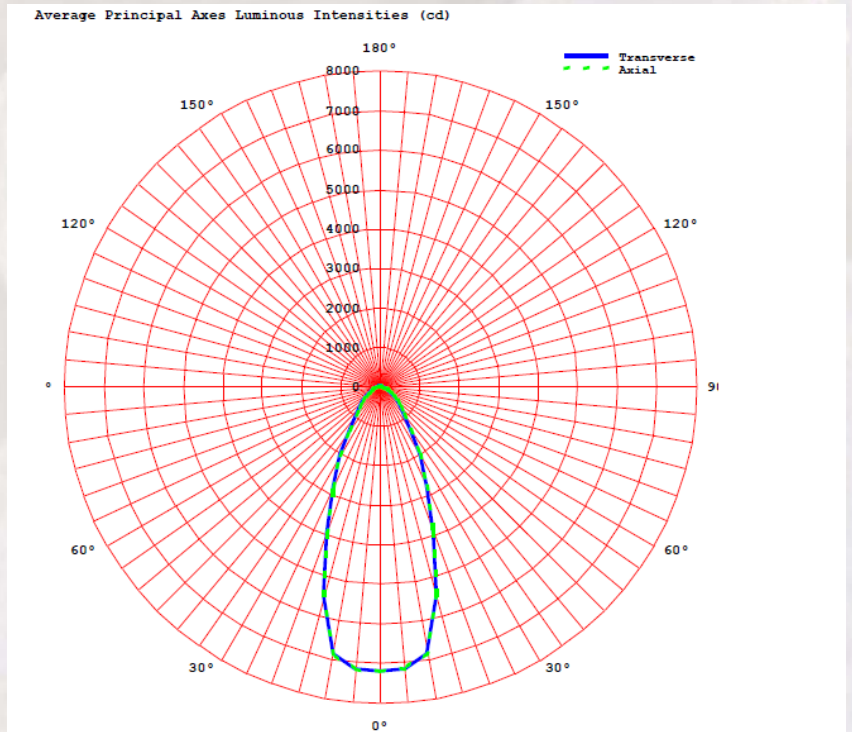
Above: Average Principal Axes Luminous Intensities (cd) - Sovereign 72XL110 – 15 DEGREE MODULE TILT
